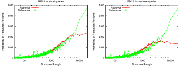
Figure 2: Comparison of retrieval and relevance probabilities against all document lengths when using BM25 on short (left) and verbose (right) queries.
