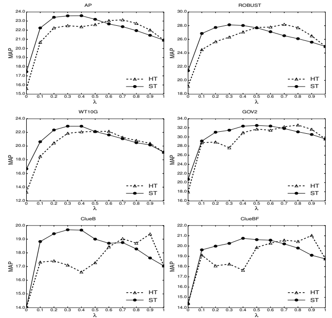
Figure 1: The effect of varying \lambda on the MAP of HT and ST. For \lambda = 1 , the methods amount to TermsLM (term-based language model retrieval). For \lambda = 0 , the methods use only entity tokens. The performance is reported for the test folds (i.e., all queries in a dataset) when fixing the value of \lambda and using cross validation to set the values of all other free parameters. Note: figures are not to the same scale.
