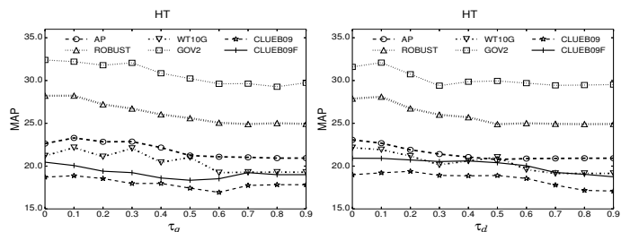
Figure 2: The effect of varying \tau_q and \tau_d on the MAP performance of HT. The values of free parameters, except for that in the x -axis, are set using cross validation as in Figure 1.
