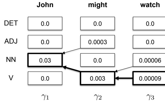
Figure 7.5: Computing the most likely state sequence that generated \langle \text{John, might, watch} \rangle under the HMM given in Figure 7.3 using the Viterbi algorithm. The most likely state sequence is highlighted in bold and could be recovered programmatically by following backpointers from the maximal probability cell in the last column to the first column (thicker arrows).
