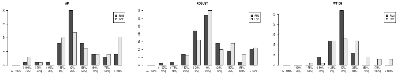
Figure 2: Histograms that demonstrate and compare the robustness of relevance models (RM3) and latent concept expansion (LCE) with respect to the query likelihood model (QL) for the AP, ROBUST, and WT10G data sets.
